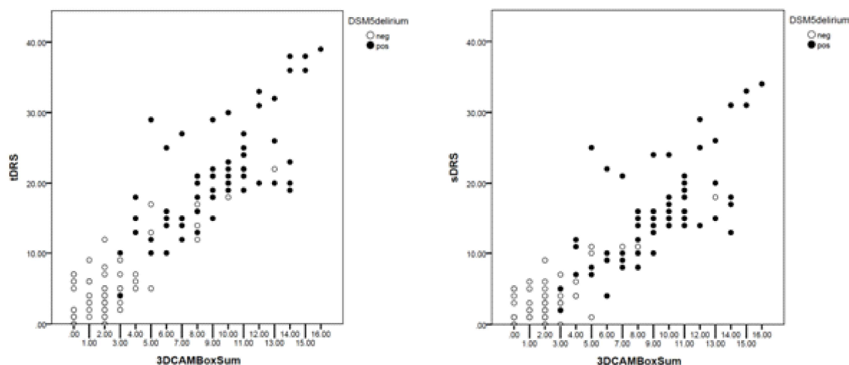
Figure 1. Scatter plot of relationship between the 3D-CAM sum of positive items and DRS- R-98 total and severity scores (3DCAMBoxSum= 3D-CAM sum of positive items; tDRS= Thai DRS-R-98 total score; sDRS= Thai DRS-R-98 severity score).
