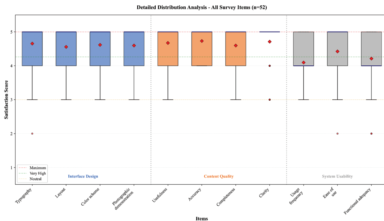
Figure 3 Distribution of satisfaction scores for the 11 questionnaire items across three dimensions: interface design, content quality, and system usability (n = 52). Box plots illustrate score distributions for each item, including the median, mean, interquartile range, and overall score range. Dashed lines indicate the maximum score (5.0), the very high satisfaction threshold ( \geq 4.26 ), and the neutral level (3.0). All items showed high satisfaction, with content accuracy having the highest mean score and usage frequency the lowest.
