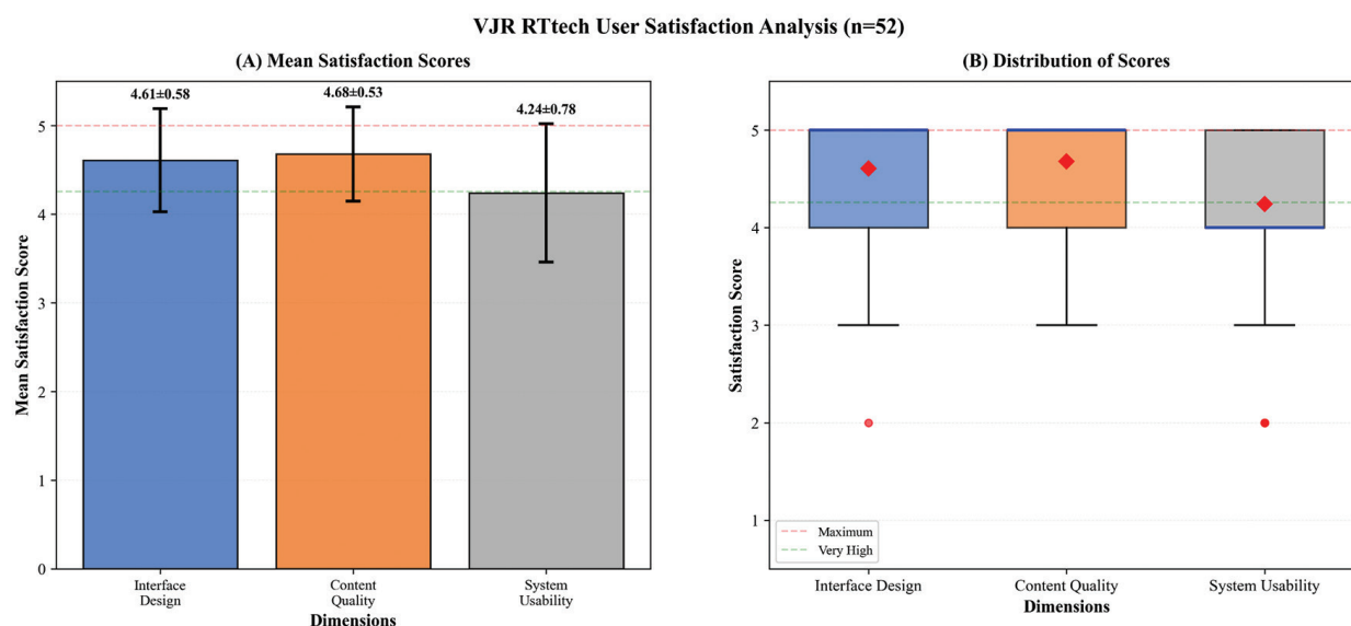
Figure 2 User satisfaction across interface design, content quality, and system usability (n = 52). (A) Mean satisfaction scores (mean ± SD) for each evaluation dimension. The red dashed line indicates the maximum score (5.0), and the green dashed line represents the threshold for very high satisfaction ( \geq 4.26 ). (B) Box plots showing score distributions across dimensions, demonstrating high to very high satisfaction, with content quality showing the highest median score.
